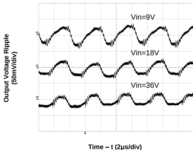
Figure 3. Output Ripple Voltage at Full Load
