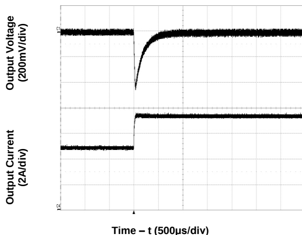
Figure 6. Transient Load Response (typical Vin, load current steps from 50% to 75% at a slew rate 0.1A/µs)
