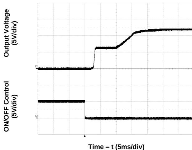
Figure 4. Start-Up from Enable Control (typical Vin, full load)
