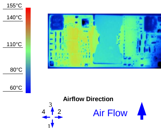
Figure 8. Thermal Image for Airflow Direction 3 (9.9A output, 55°C ambient, 200 LFM, typical Vin, open frame, unit soldered onto a fixture board)
