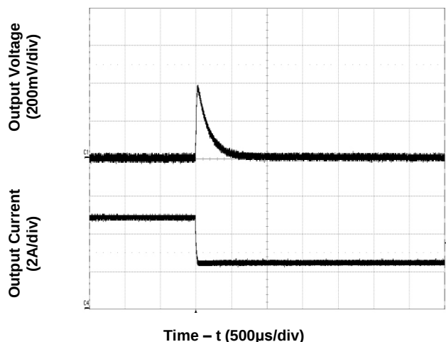
Figure 5. Transient Load Response (typical Vin, load current steps from 50% to 25% at a slew rate 0.1A/µs)
